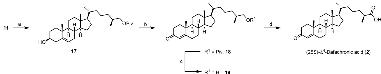
Scheme 3. Synthesis of (25 S )- \Delta^4 -dafachronic acid ( 2 ). Reagents and conditions : (a) 1.5 equiv. TBAF, THF, reflux, 17 h, 92%; (b) 1.5 equiv. Al(O i Pr) 3 , acetone/toluene (1:9), 100 °C, 5 h, 86%; (c) 2.0 equiv. NaOMe, MeOH, 25 °C, 5 d, 56% of 19 , 15% of 18 ; (d) 5.0 equiv. Jones reagent, 0 °C, 90 min, 65%.
