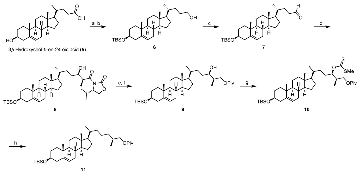
Scheme 1. Stereoselective synthesis of the crucial intermediate 11 . Reagents and conditions : (a) 3.2 equiv. TBSCl, 8.1 equiv. imidazole, 2.2 equiv. DMAP, DMF, 25 °C, 18 h; (b) 4.0 equiv. LiAlH 4 , THF, 25 °C, 17 h, 96% for 2 steps; (c) 4.0 equiv. DMSO, 2.0 equiv. (COCl) 2 , CH 2 Cl 2 , –78 °C, then 6 , 20 min, 5.0 equiv. Et 3 N, to 25 °C, 98%; (d) 1.3 equiv. ( S )-(+)-4-isopropyl-3-propionyl-2-oxazolidinone, 1.43 equiv. Bu 2 BOTf, 1.69 equiv. Et 3 N, CH 2 Cl 2 , 0 °C, 1 h, then –78 °C, 7 , 30 min, then 0 °C, 80 min, 95%; (e) 1.1 equiv. LiBH 4 , 1.0 equiv. H 2 O, Et 2 O, 0 °C, 2 h; (f) 1.3 equiv. PivCl, pyridine/CH 2 Cl 2 (1:1), 0 °C, 2 h, 81% for 2 steps; (g) 1.0 equiv. NaHMDS, 20.0 equiv. CS 2 , THF, –78 °C to 0 °C, then 2.0 equiv. MeI, 30 min, 98%; (h) 10 mol-% AIBN, 15.0 equiv. Bu 3 SnH, reflux, 5 min, 93%.
